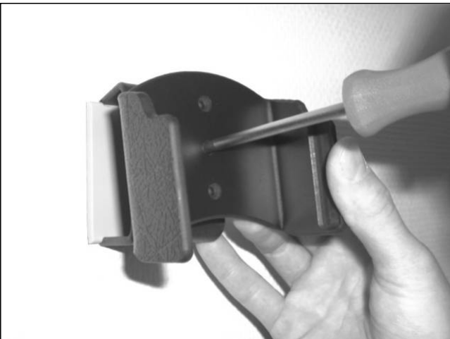
3. Start to thread the center screw into the base plate. When you connect with the nut pull the holder towards you to prevent the nut from spinning around. Continue to tighten the screw firmly. Then loosen the screw slightly for easier angling/rotation of the holder.
