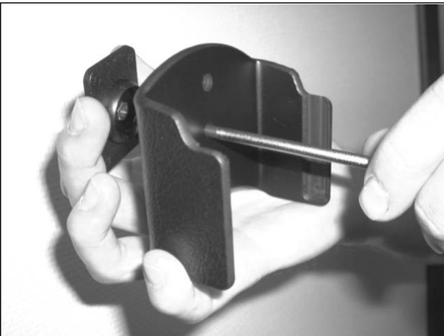
1. Unscrew the screw in the center of the holder and remove the holder from the Tilt Swivel base plate.
